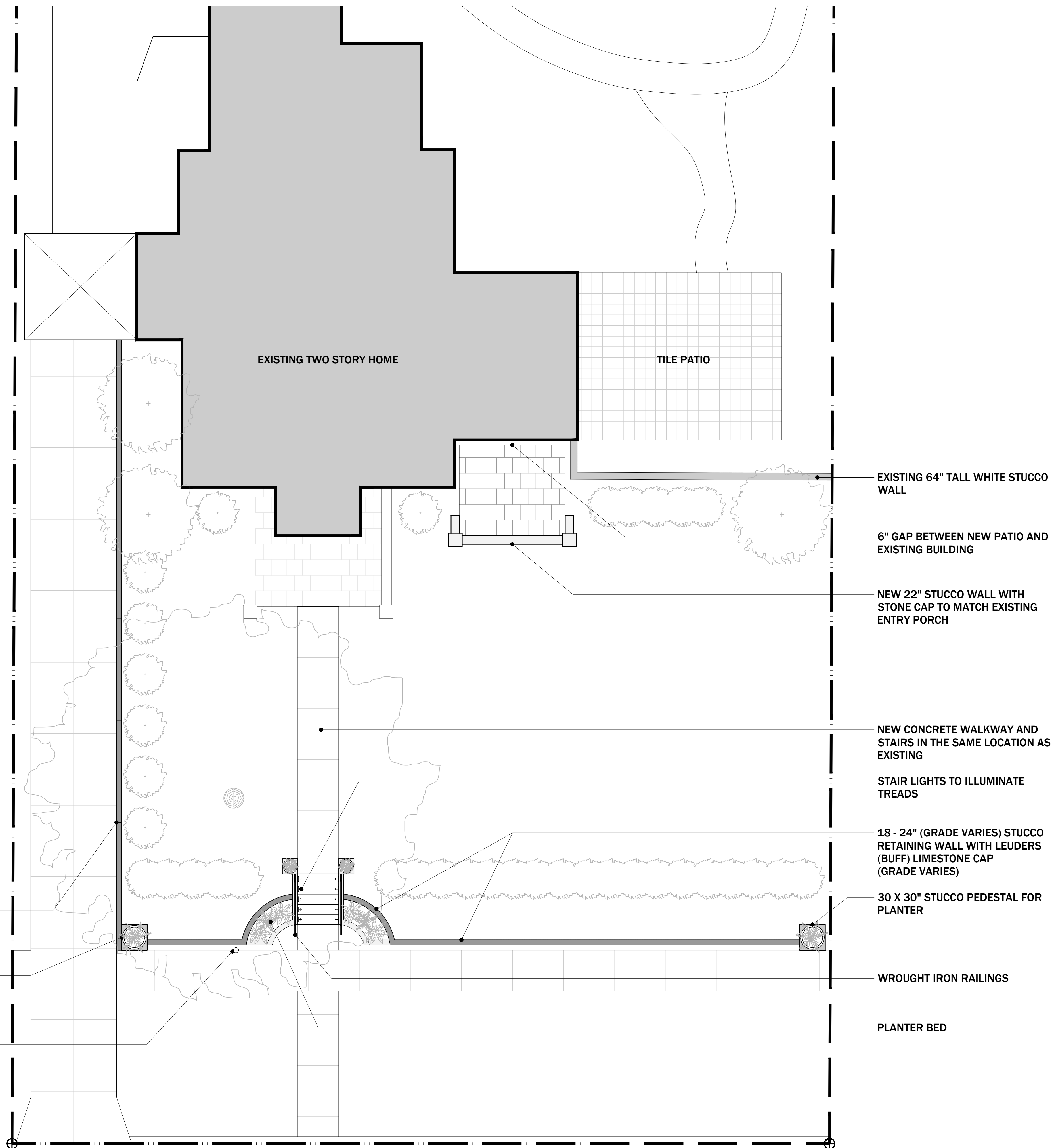
1 LANDSCAPING PLAN SCALE: 3/16" = 1'-0"
