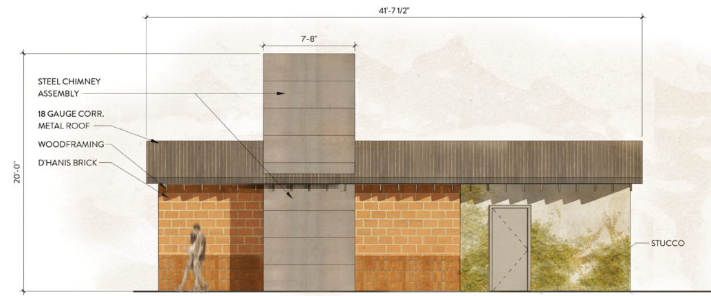
5 FOOD SERVICE - NORTH ELEVATION
