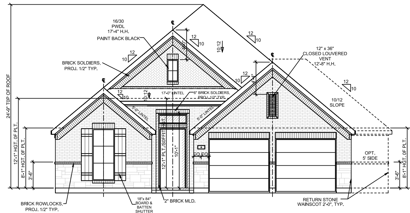
1 FRONT ELEVATION @ E-31 1/8" = 1'-0"
