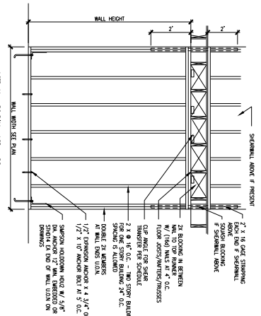
TYPICAL BRACED WALL DETAIL NO SCALE
