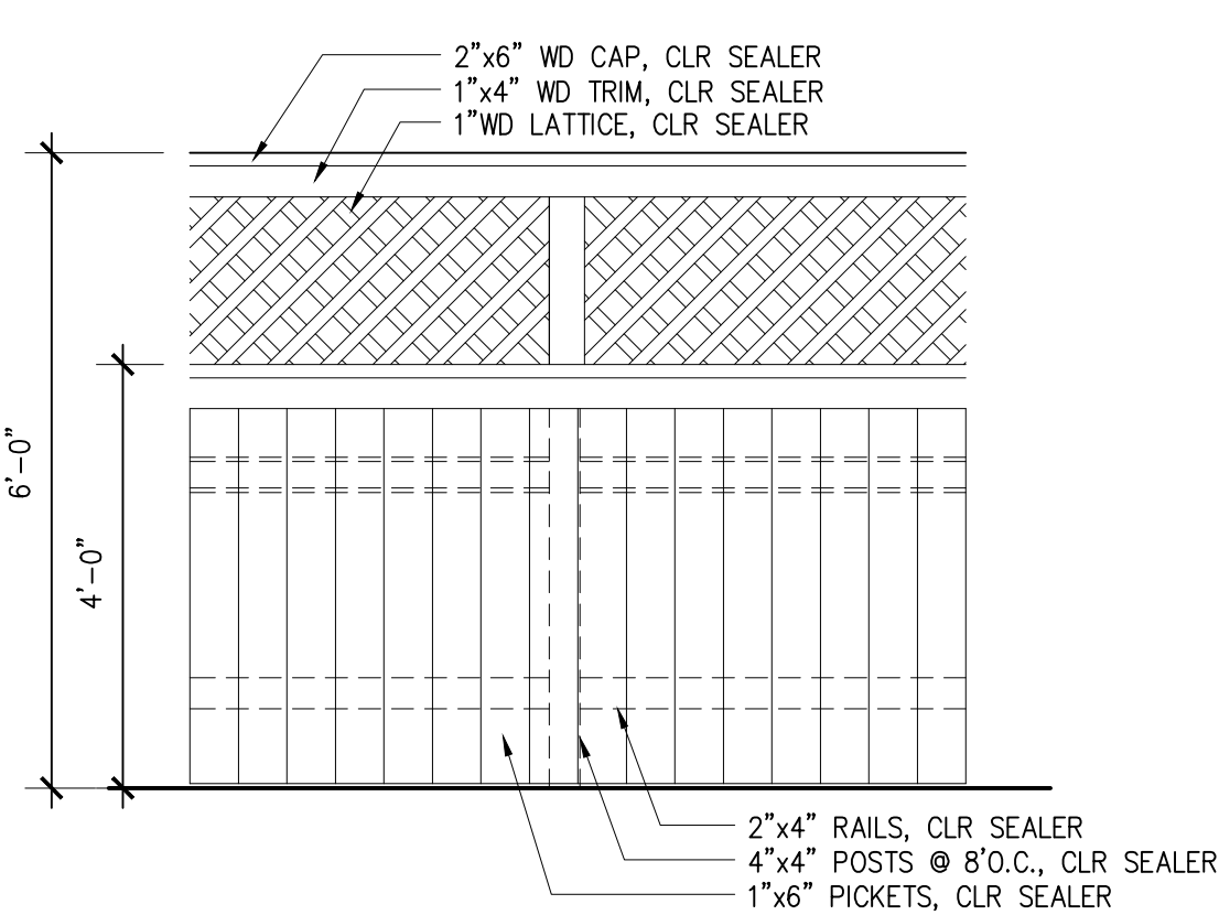
2 ELEVATION: 6'-0" WOOD PRIVACY FENCE SCALE: 1/2" = 1'-0"
