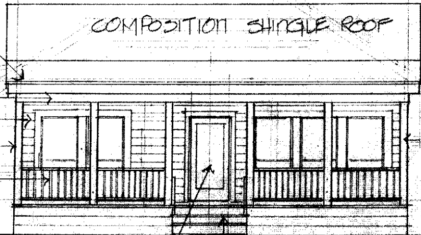
1/4 FRONT ELEVATION
