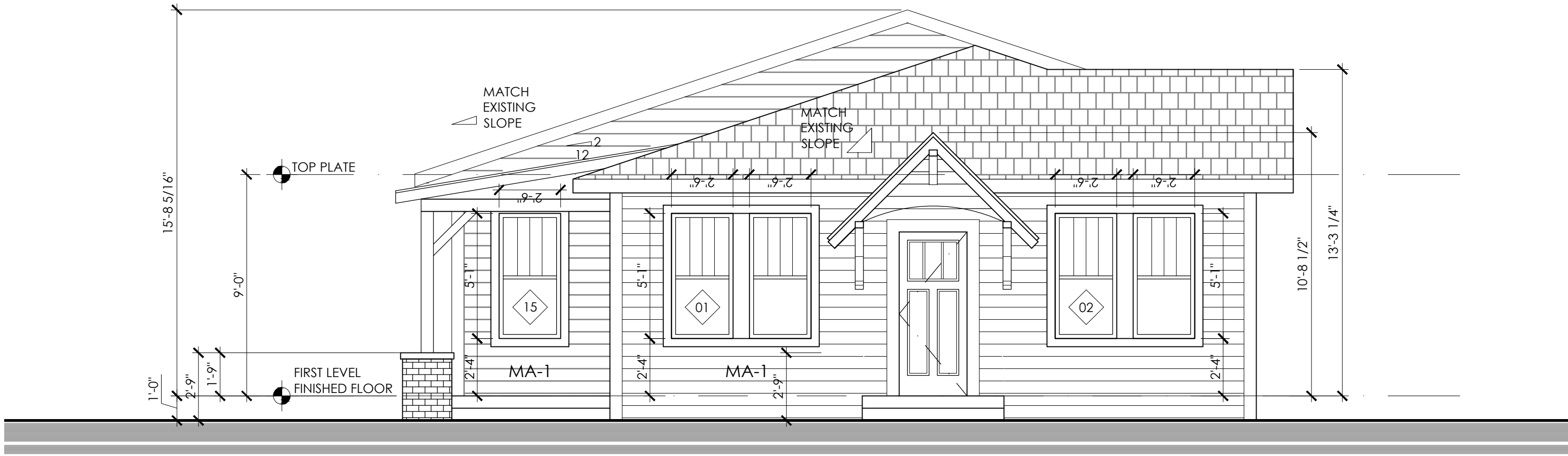
N EXTERIOR ELEVATION 1/4" = 1'-0"
