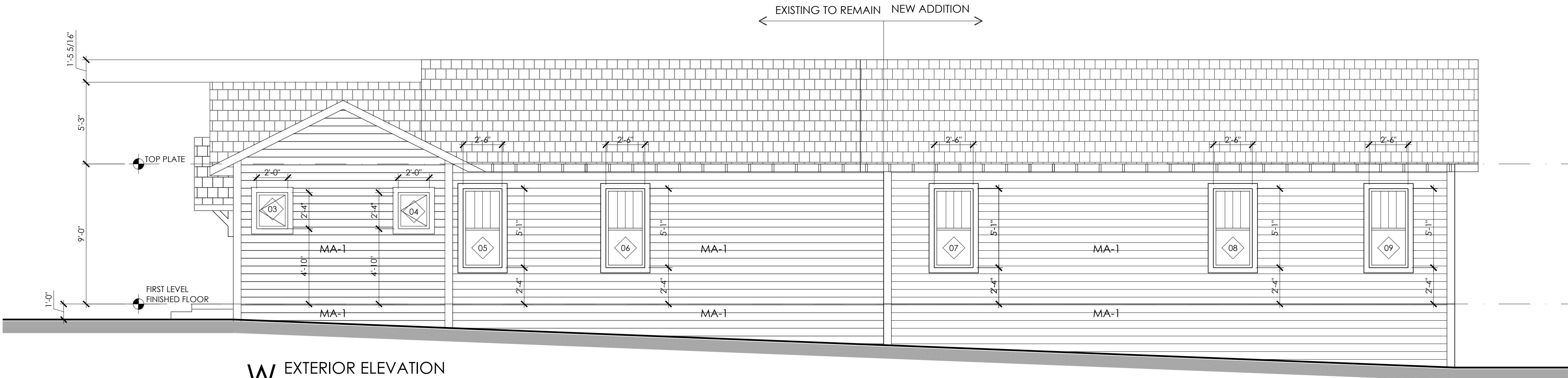
W EXTERIOR ELEVATION 1/4" = 1'-0"
