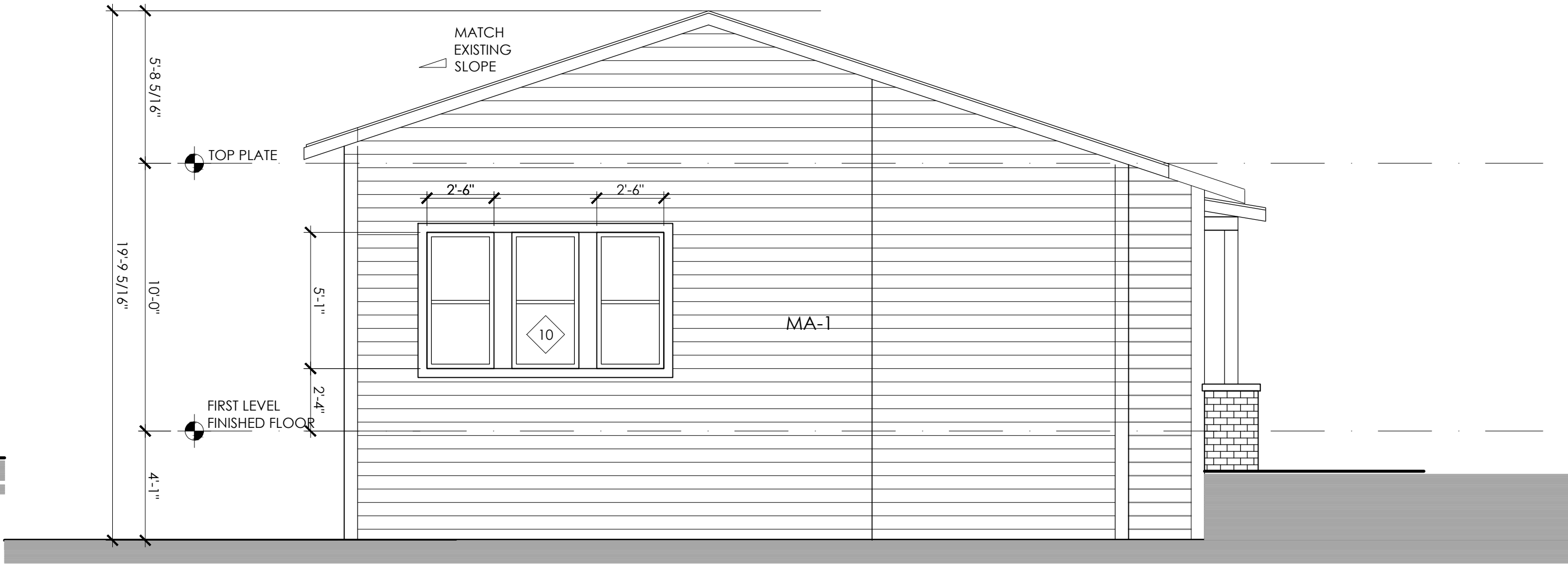
S EXTERIOR ELEVATION 1/4" = 1'-0"
