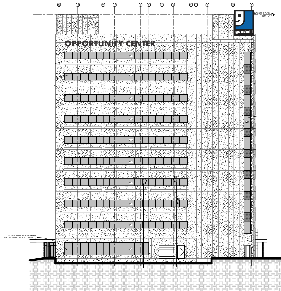
3 EXTERIOR ELEVATION 1/8" = 1'-0"
