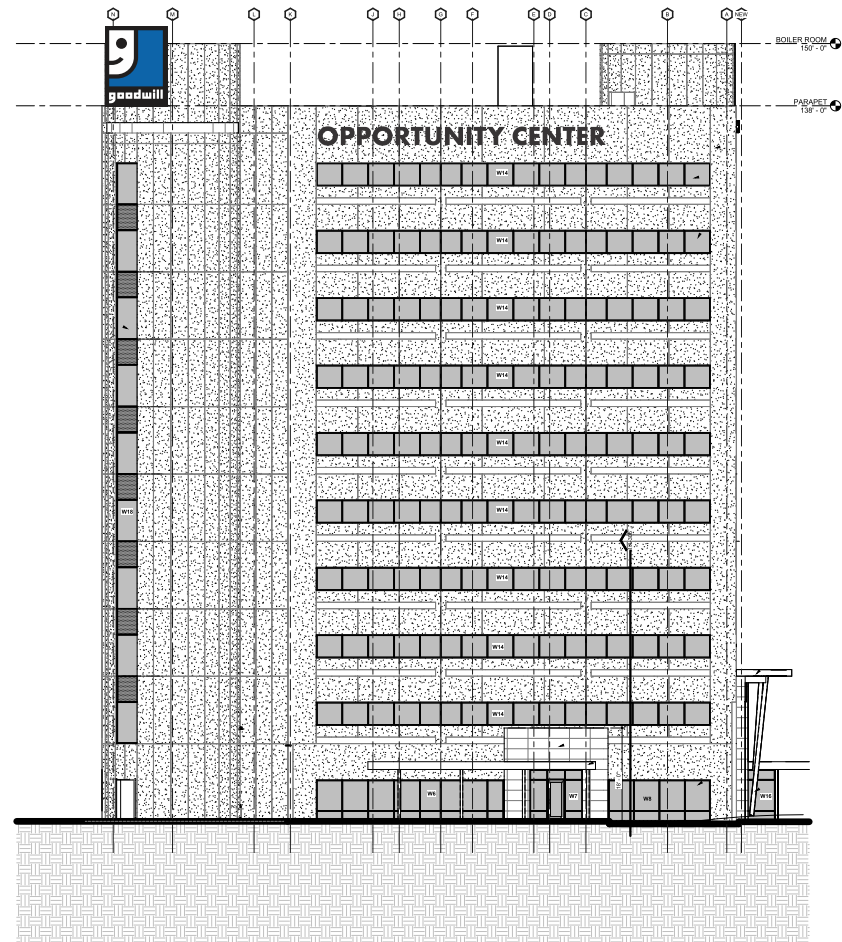
1 EXTERIOR ELEVATION 1/8" = 1'-0"
