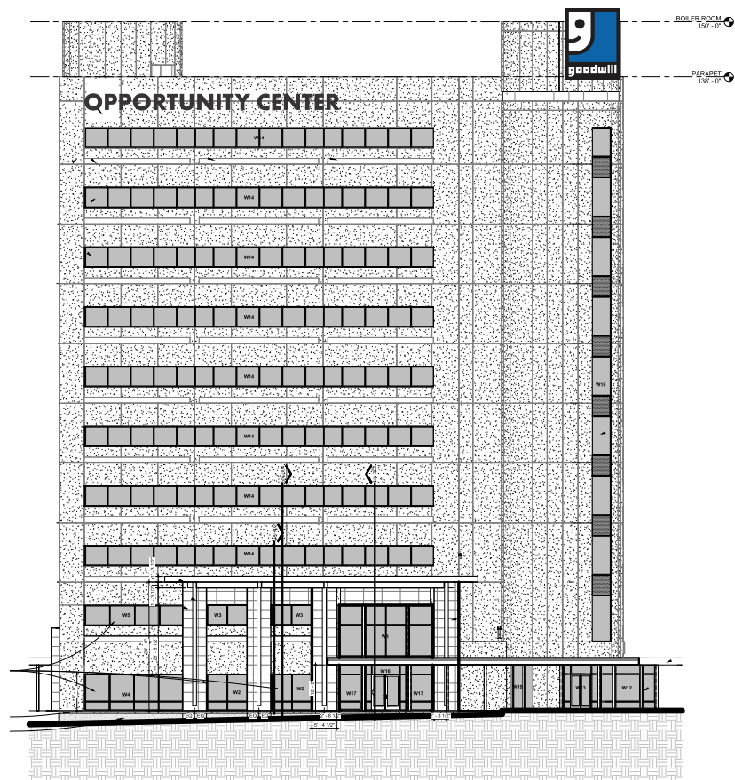
1 EXTERIOR ELEVATION 1/8" = 1'-0"
