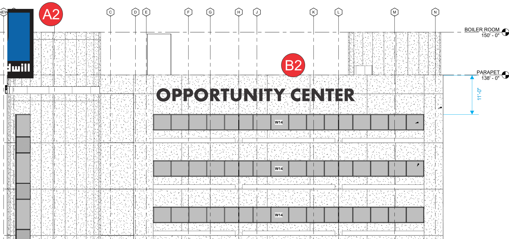
EAST ELEVATION - SCALE: 1/16"=1'-0"
