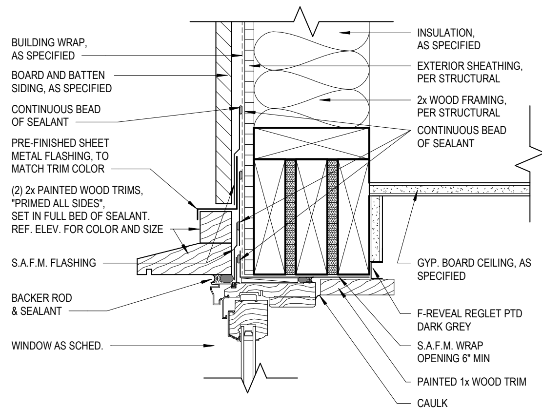
TYP. WINDOW HEAD DETAIL
