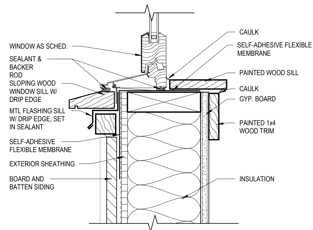
TYP. WINDOW SILL DETAIL
