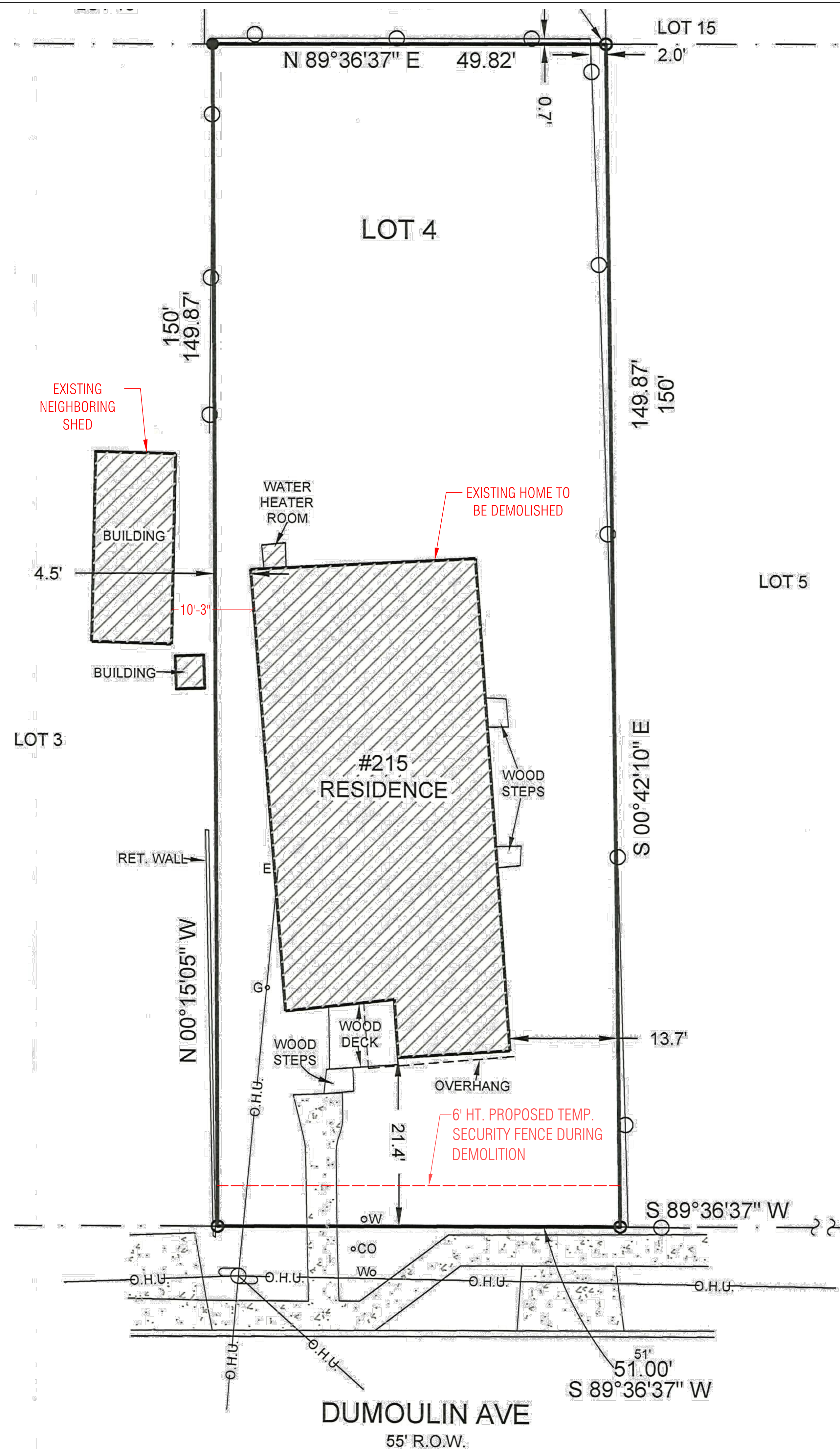
EXISTING SITEPLAN LAYOUT
