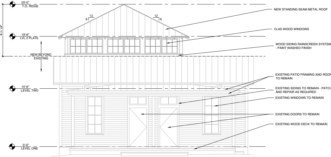
EXTERIOR ELEVATION - SOUTH 01 1/4" = 1'-0"
