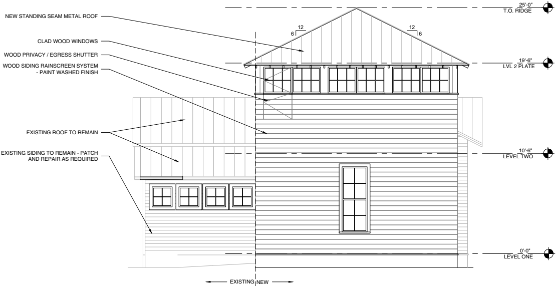
EXTERIOR ELEVATION - NORTH 03 1/4" = 1'-0"
