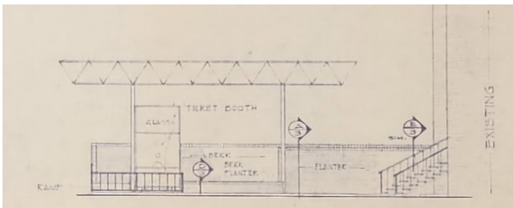
East Elevation of Canopy for HemisFair, 1967
