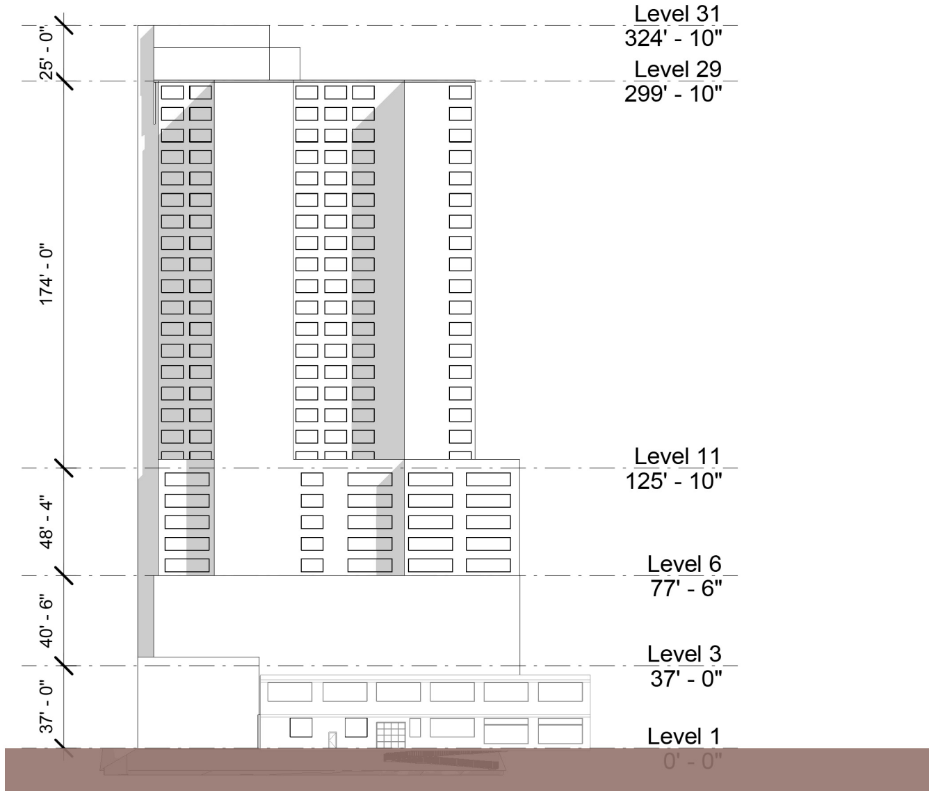
PROPOSED ELEVATION MASSING - NORTH
