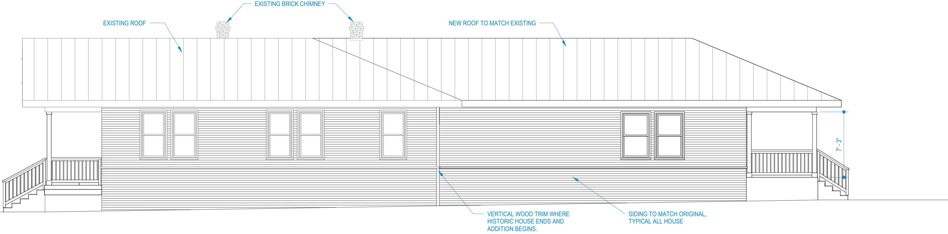
2 West 3/16" = 1'-0"
