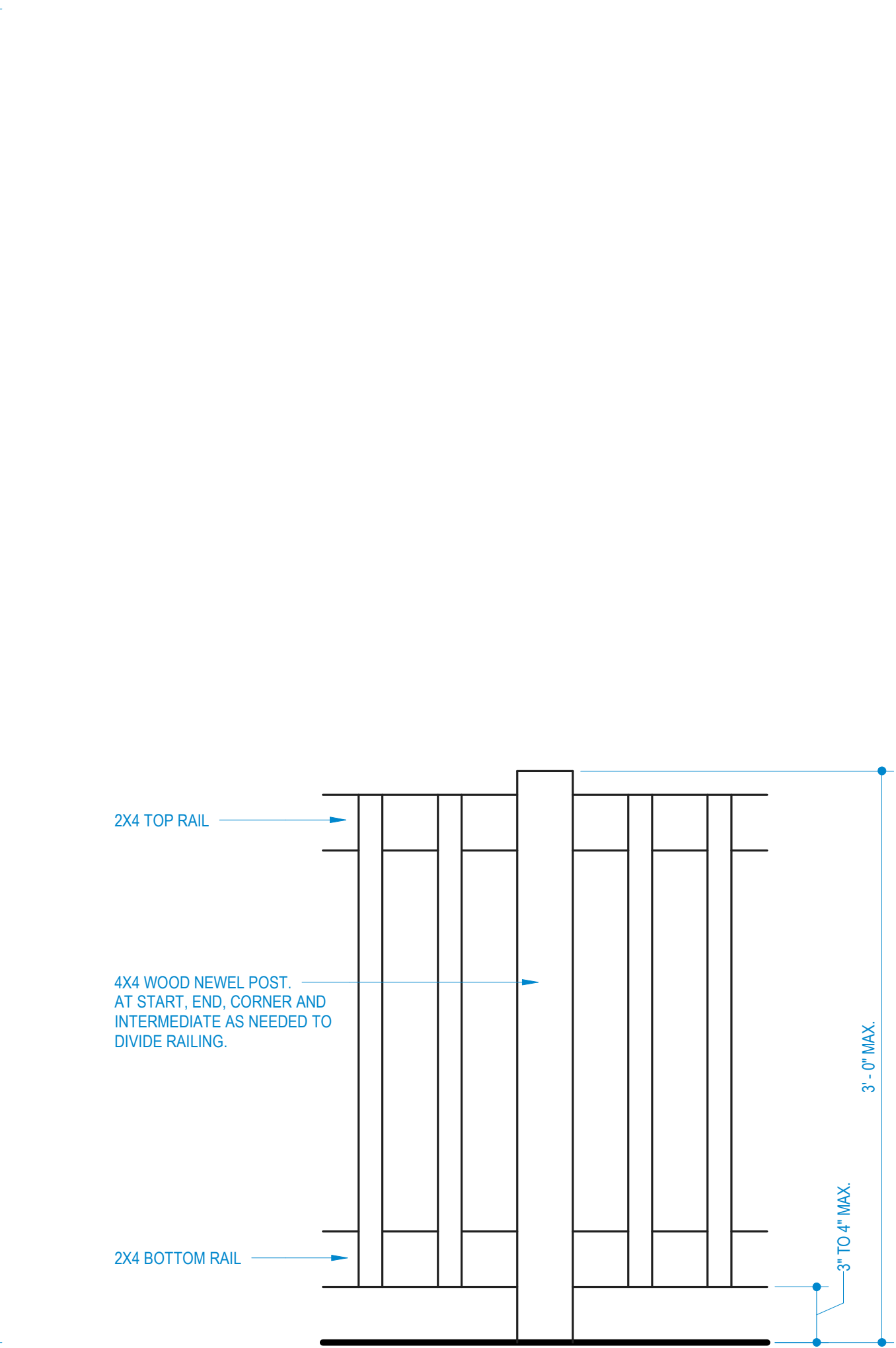
2 RAILING DETAIL 1 1/2" = 1'-0"
