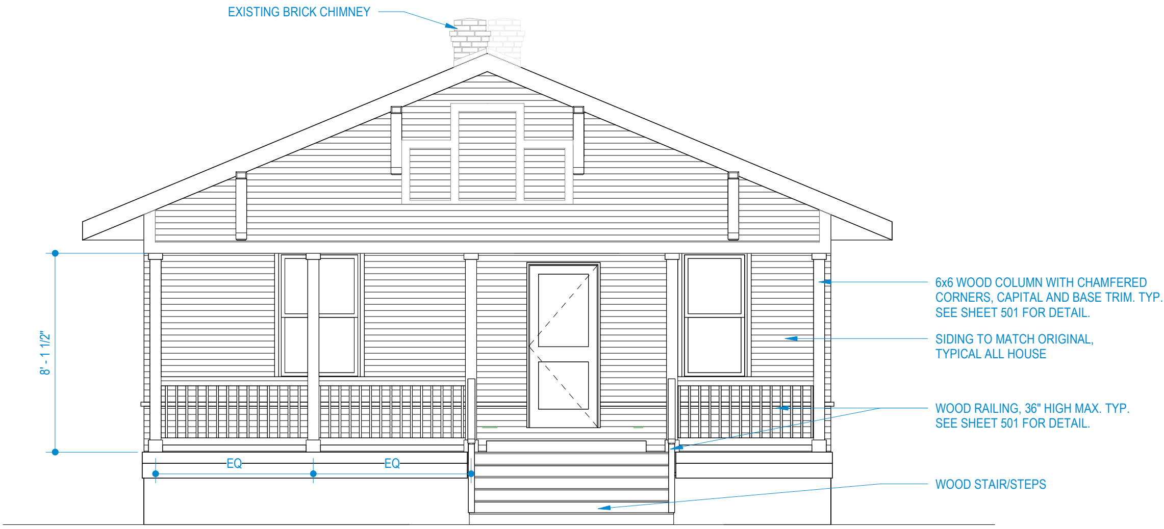
1 North 1/4" = 1'-0"
