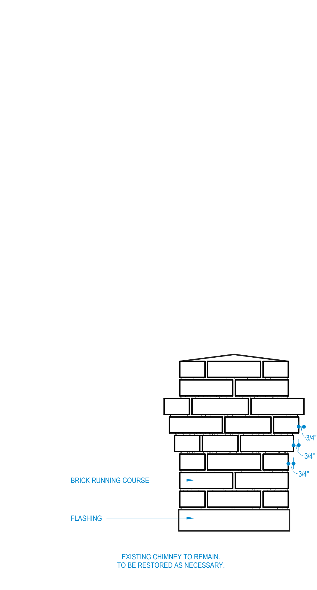
3 EXISTING CHIMNEY 1 1/2" = 1'-0"
