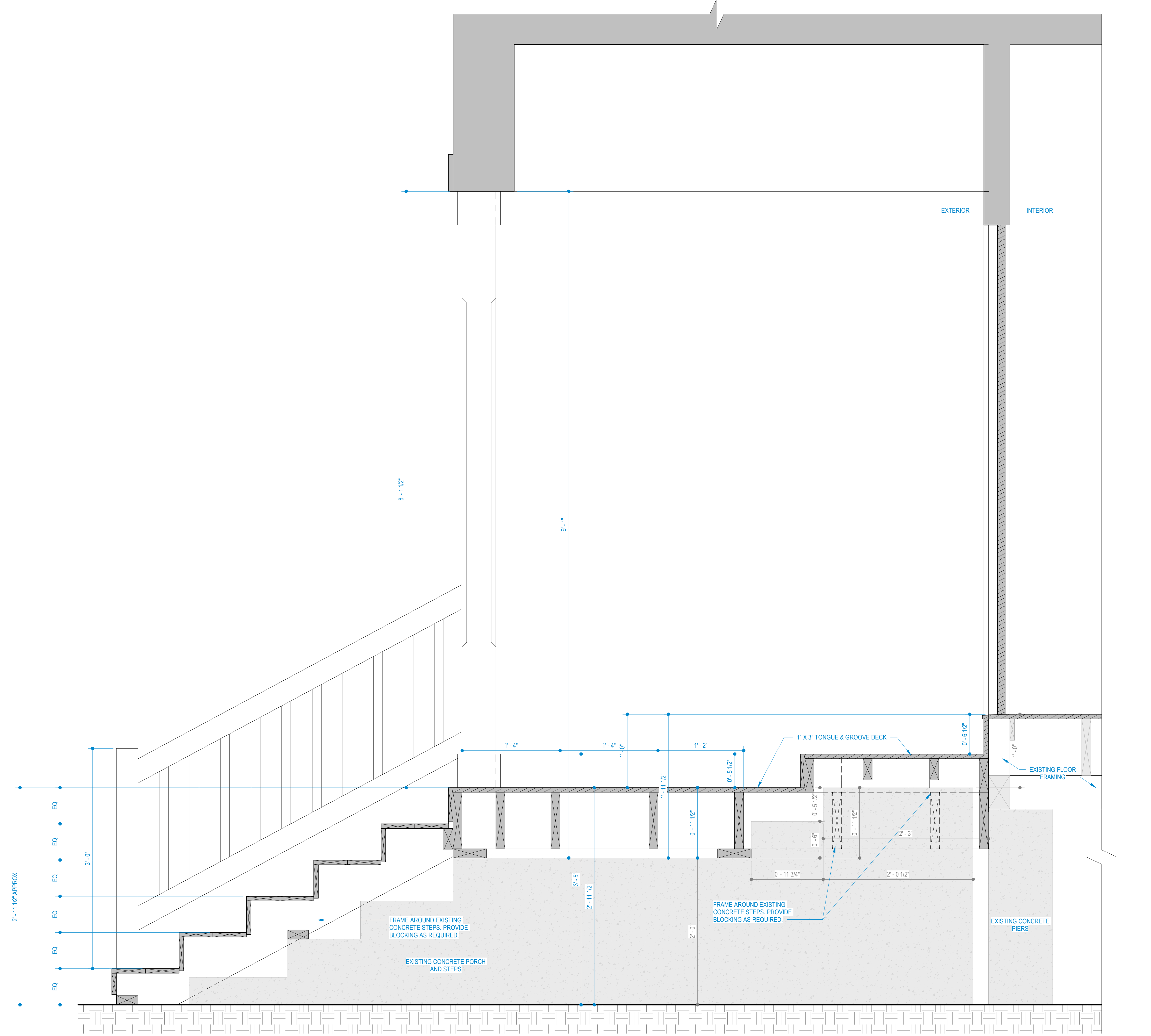
4 ENTRY PORCH SECTION 1 1/2" = 1'-0"
