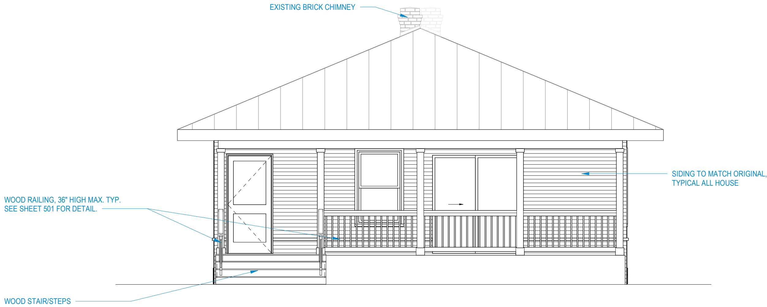
3 South 1/4" = 1'-0"
