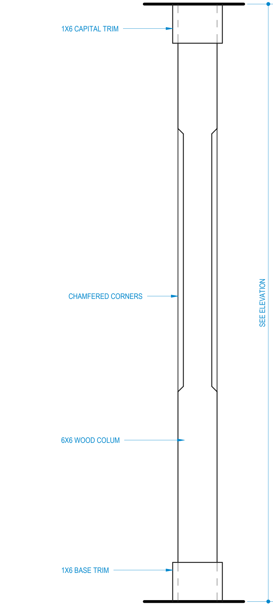
1 COLUMN DETAIL 1 1/2" = 1'-0"
