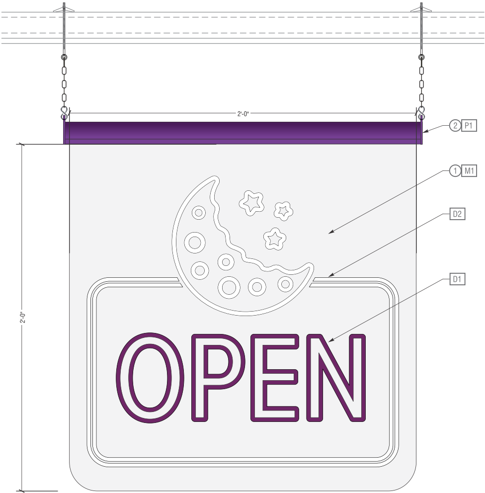
illuminated edge-lit hanging window sign Scale : 1 1/2" = 1'-0"
