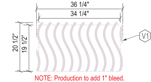
Window Vinyl 2 Layout QTY 1 Scale: 1/2" = 1'-0"
