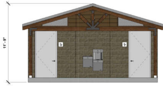
Proposed Pre-Fabricated Restroom Building
