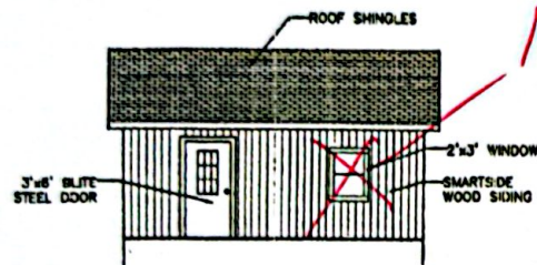
SIDE WALL ELEVATION WITH OPENINGS
