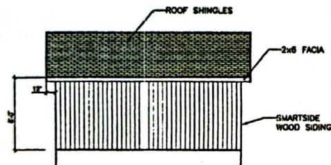
BLANK SIDE WALL ELEVATION
